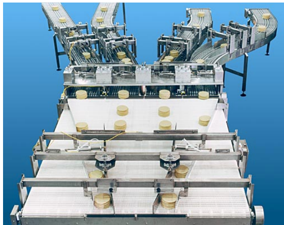
4 : 2 Pizza Crust Merge
