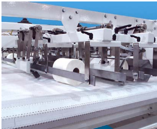
Mat Top / Squeeze Gate
