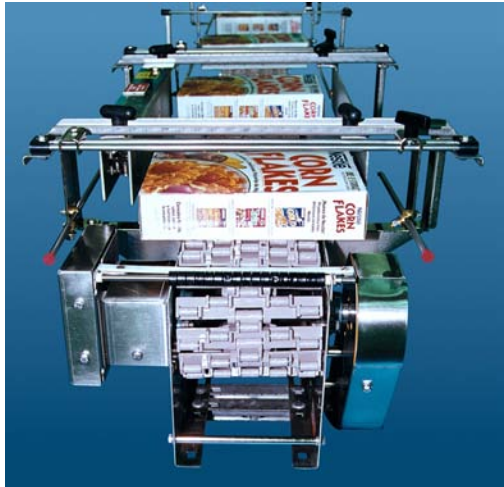
Low Back Pressure Table Top
