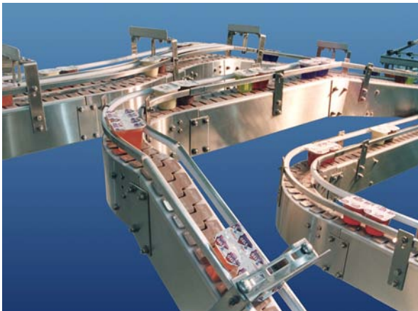
Cups on 4 Lane Table Top
