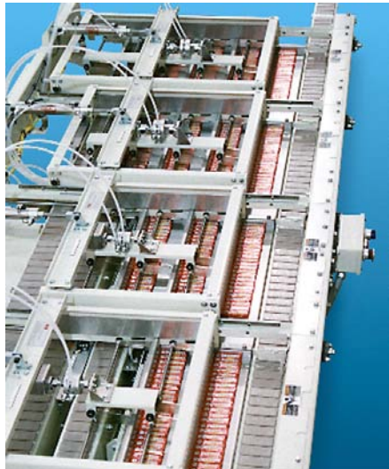
Hi Speed 5 : 1 Merge 1200 PPM
